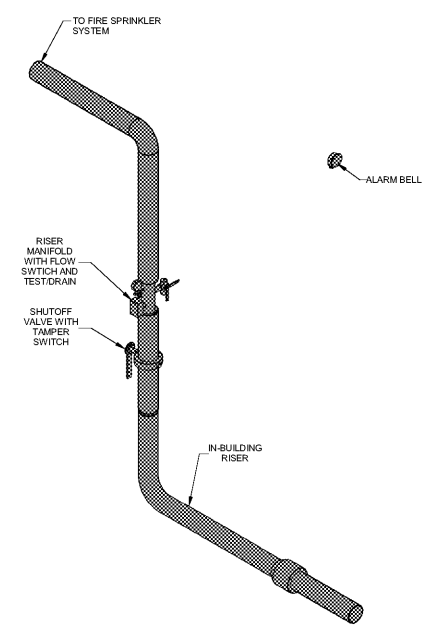
3 FIRE SPRINKLER SERVICE RISER F3.01 NOT TO SCALE
