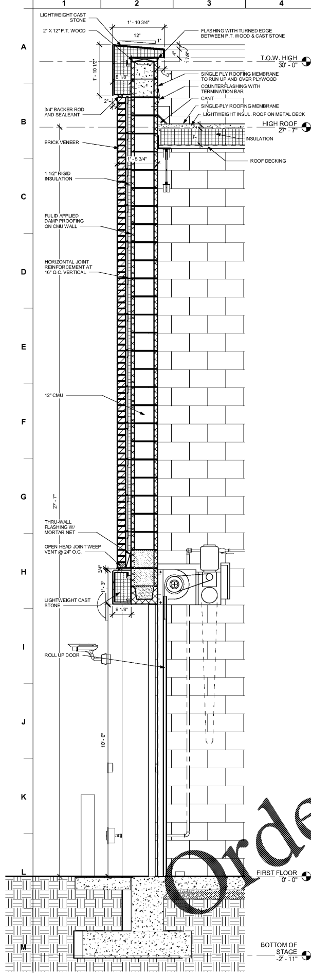
3 Detail 11 3/4" = 1'-0"
