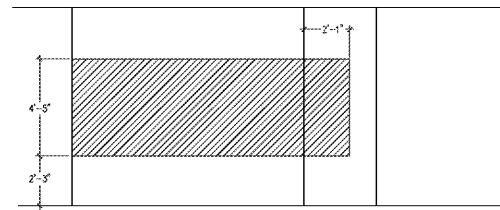
2 PREP AREA WALL BACKING
