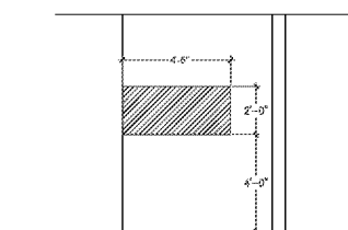
4 SIDE PREP AREA WALL BACKING
