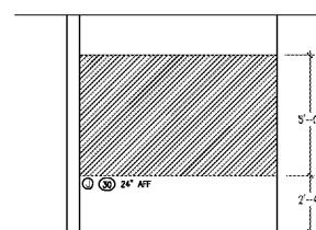
1 POT WASH / PREP AREA WALL BACKING
