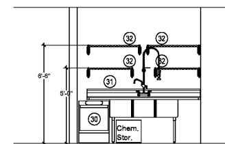
1 POT WASH / PREP AREA
