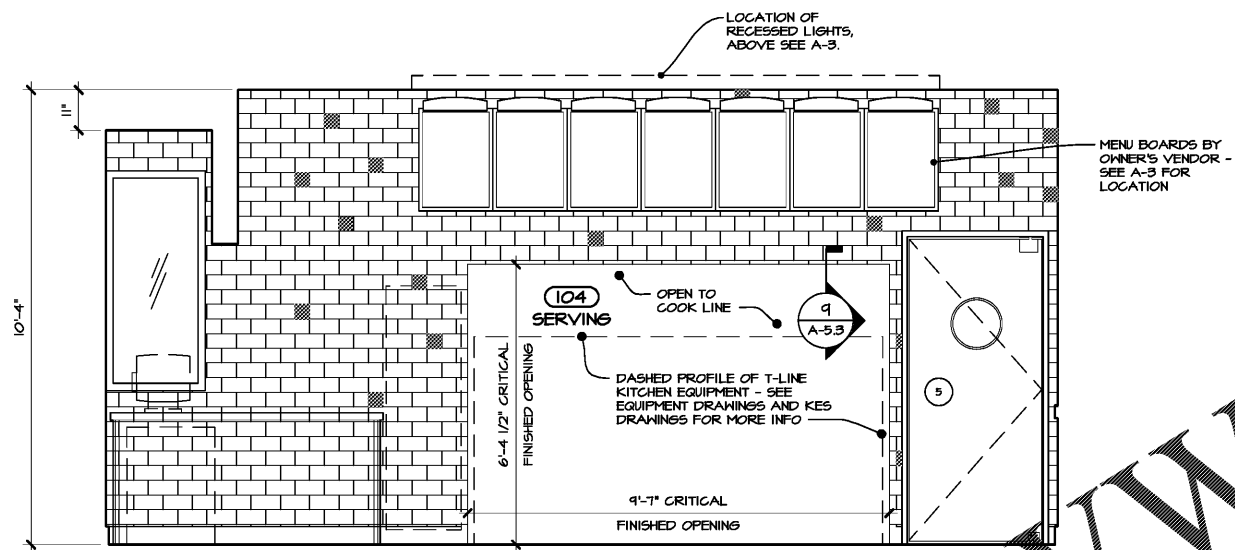
1 VESTIBULE AND SERVICE COUNTER - MENU BOARD PLACEMENT A-8.2 SCALE 1/2" = 1'-0"
