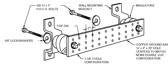
3 GROUNDING BAR DETAIL E.402 NO SCALE
