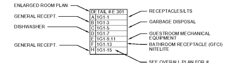
3 GUESTROOM CIRCUIT KEY E 202 NO SCALE
