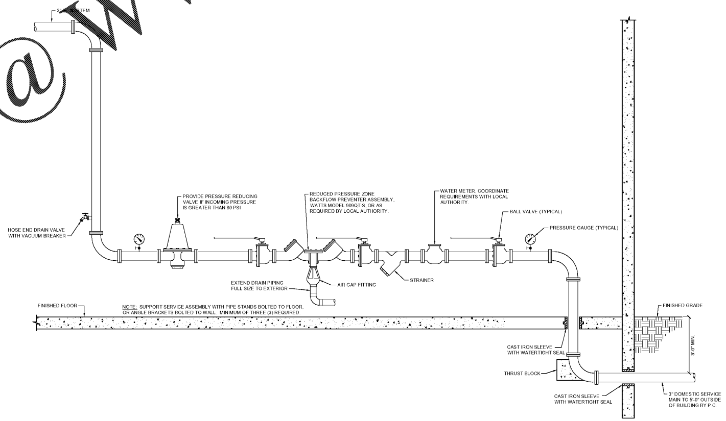
1 DOMESTIC SERVICE ENTRANCE DETAIL P.004 NOT TO SCALE
