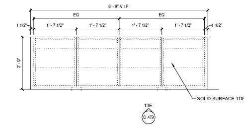
13A PLAN - BOARD ROOM SCALE: 3/4" = 1'-0"
