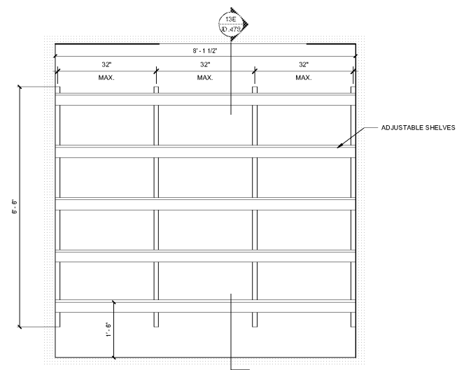
13A ELEVATION - HOUSE LAUNDRY SCALE: 3/4" = 1'-0"
