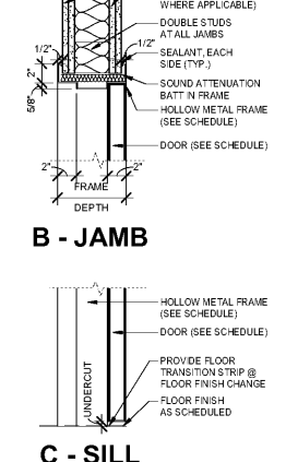
DOOR DETAILS S4 FOR WALL TYPES "S4"
