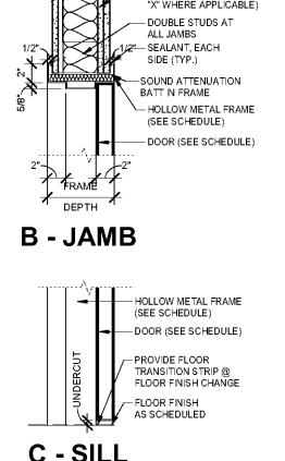
DOOR DETAILS S3 FOR WALL TYPES "S3"
