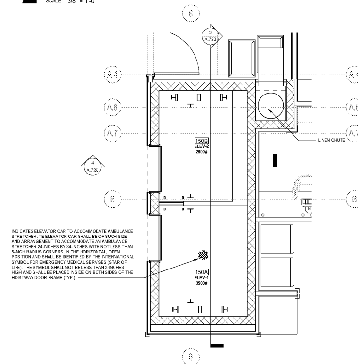
ENLARGED PLAN - ELEVATOR LOBBY 1ST 1 FLOOR SCALE: 3/8" = 1'-0"
