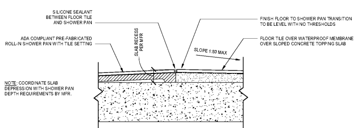
1 TRANSITION @ ROLL-IN SHOWER SCALE: 3" = 1'-0"
