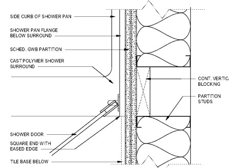
6 SHOWER CORNER PLAN DETAIL SCALE: 3" = 1'-0"
