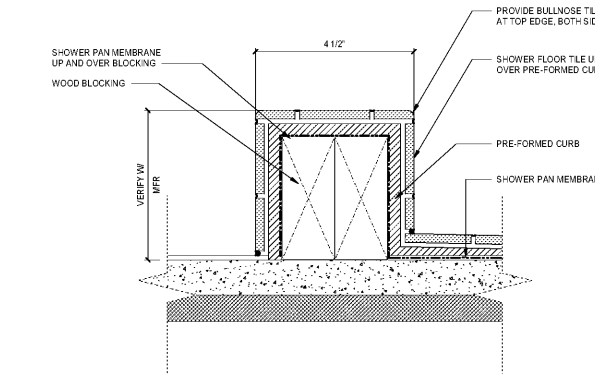
2 SHOWER CURB DETAIL SCALE: 6\"/>
