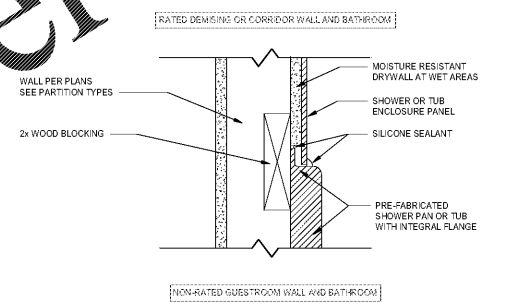
7 SHOWER/TUB BASE DETAIL SCALE: 3" = 1'-0"
