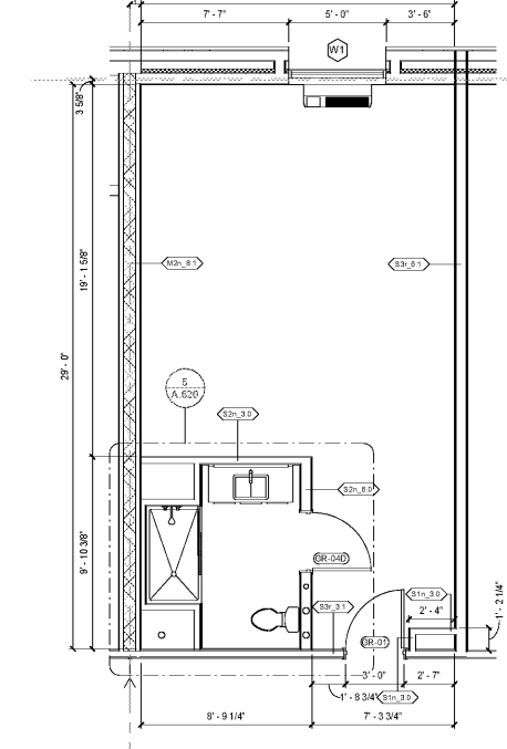
1 KING STUDIO WIDE - ARCH PLAN SCALE: 1/4" = 1'-0"
