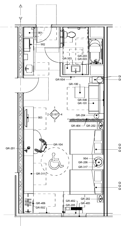
4 DBL QUEEN STUDIO ADA TUB - FF&E PLAN SCALE: 1/4" = 1'-0"
