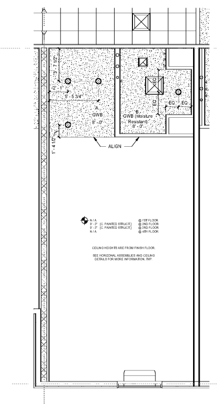
6 DBL QUEEN STUDIO ADA TUB - CEILING PLAN SCALE: 1/4" = 1'-0"
