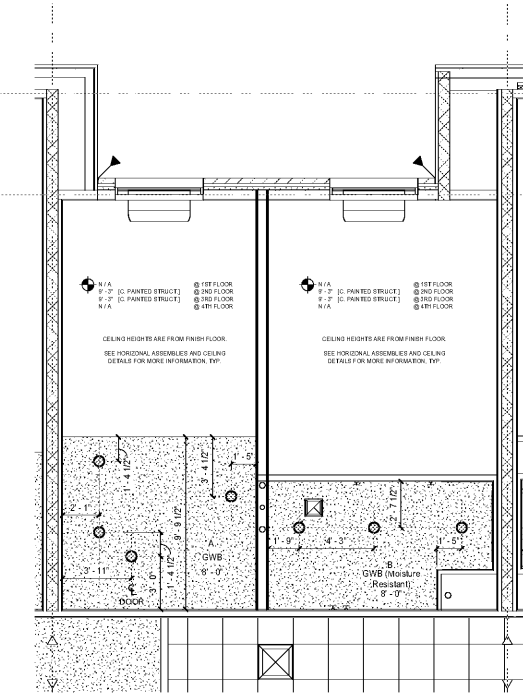
6 KING SUITE ADA TUB - CEILING PLAN SCALE: 1/4" = 1'-0"
