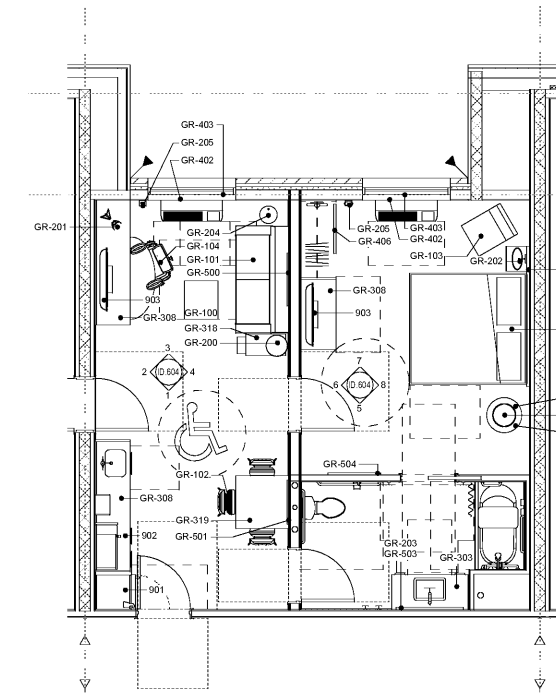
4 KING SUITE ADA TUB - FF&E PLAN SCALE: 1/4" = 1'-0"
