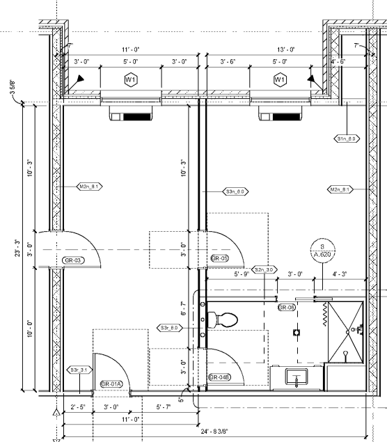
1 KING SUITE ADA RIS - ARCH PLAN SCALE: 1/4" = 1'-0"
