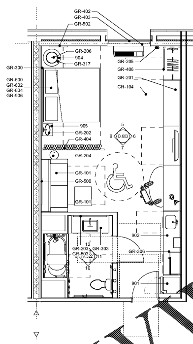
4 KING STUDIO ADA TUB - FF&E PLAN SCALE: 1/4" = 1'-0"
