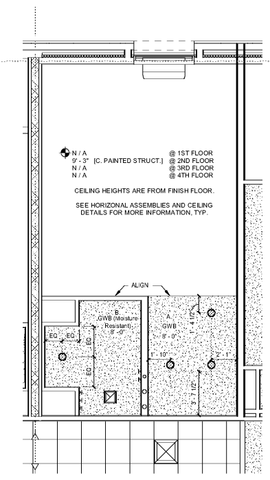
6 KING STUDIO ADA TUB - CEILING PLAN SCALE: 1/4" = 1'-0"
