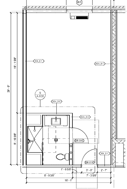
1 KING STUDIO ADA RIS - ARCH PLAN SCALE: 1/4" = 1'-0"
