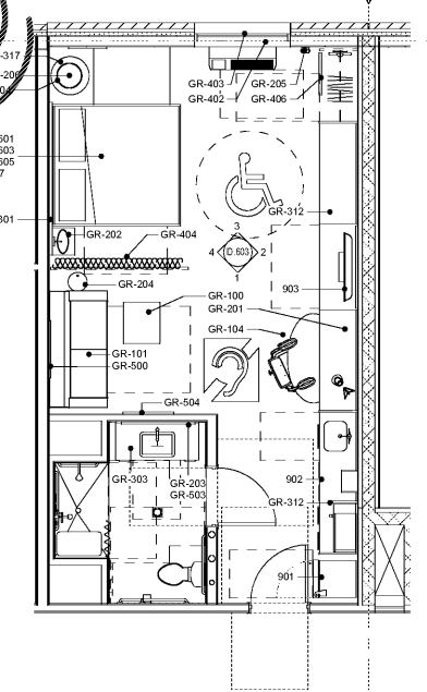
3 KING STUDIO ADA RIS - FF&E PLAN SCALE: 1/4" = 1'-0"
