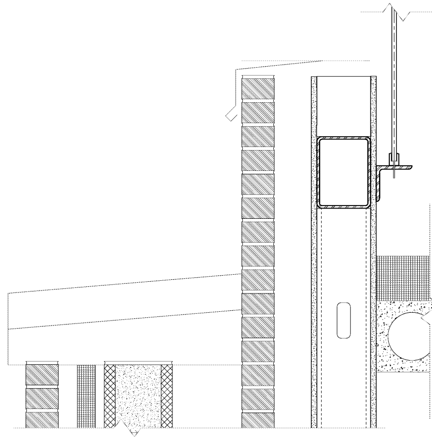
1 WSD_PARAPET - 4" BRICK, 8" CMU, 4" BRICK, 6" CFMF SCALE: 3" = 1'-0"
