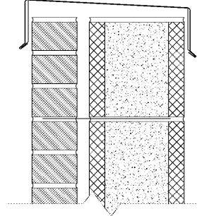
3 WSD_PARAPET - 4" BRICK, 8" CMU, PATIO SCALE: 3" = 1'-0"
