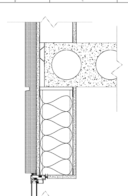
WSD WALL - 2" EIFS, 6" CFMF, PTAC HEAD SCALE: 3" = 1'-0"
