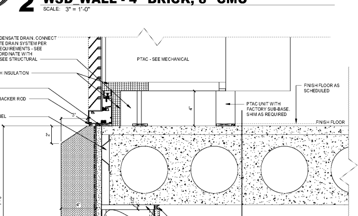
WSD WALL - 4" BRICK, 8" CMU SCALE: 3" = 1'-0"
