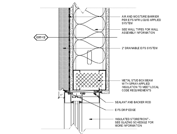
WSD WALL - 2" EIFS, 6" CFMF, STOREFRONT HEAD SCALE: 3" = 1'-0"
