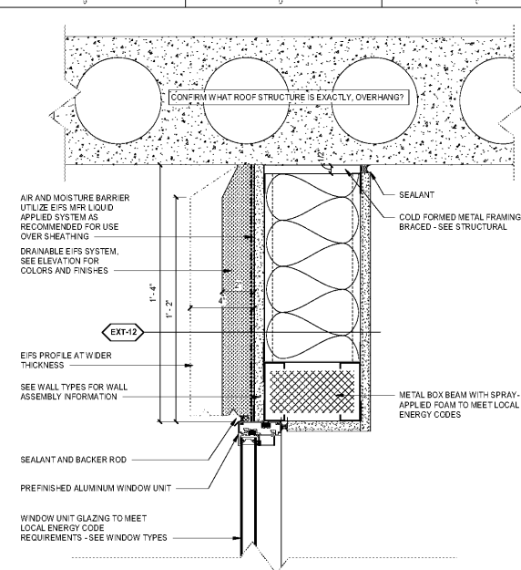
WSD WALL - 2" EIFS, 6" CFMF, PTAC HEAD AT OVERHANG SCALE: 3" = 1'-0"
