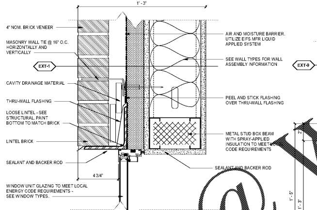
WSD WALL - 4" BRICK, 6" CFMF, PTAC HEAD SCALE: 3" = 1'-0"
