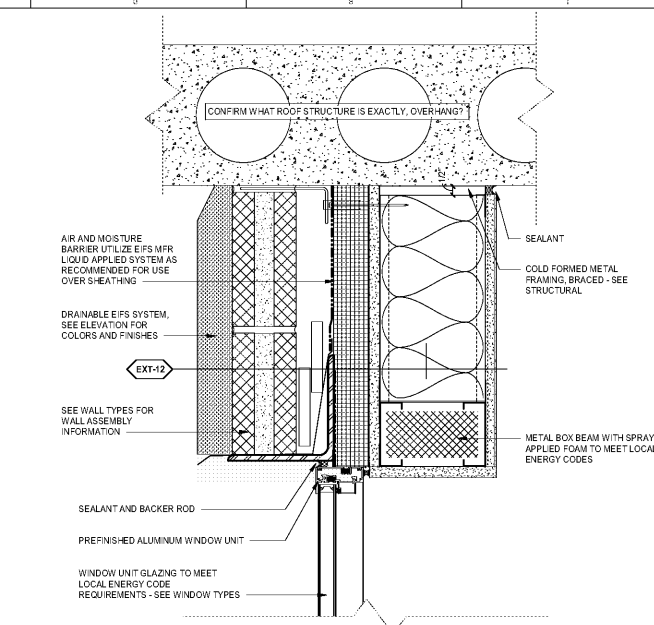
WSD WALL - 2" EIFS, 4" BRICK, 6" CFMF, PTAC HEAD AT OVERHANG SCALE: 3" = 1'-0"
