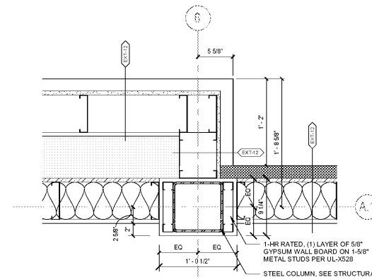
10 PD 1ST FLR TYP LINEN CHUTE SCALE: 1 1/2" = 1'-0"
