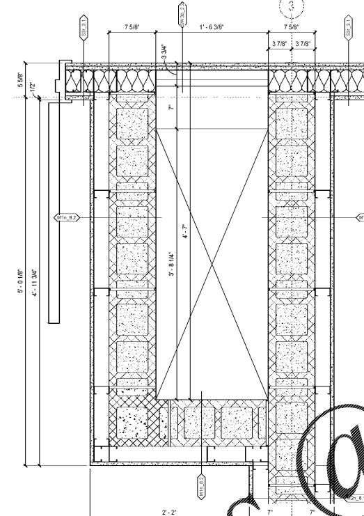
7 PD 1ST FLR 3 & E 6 SCALE: 1 1/2" = 1'-0"
