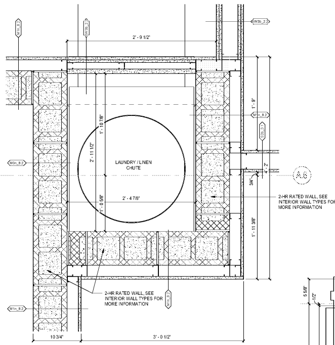
10 PD 1ST FLR TYP LINEN CHUTE SCALE: 1 1/2" = 1'-0"
