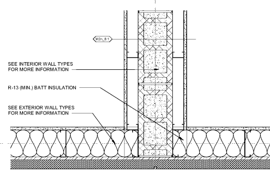
6 PD 2ND FLR TYP BLOCK TERMINATION @ EXTERIOR (EIFS) SCALE: 1 1/2" = 1'-0"
