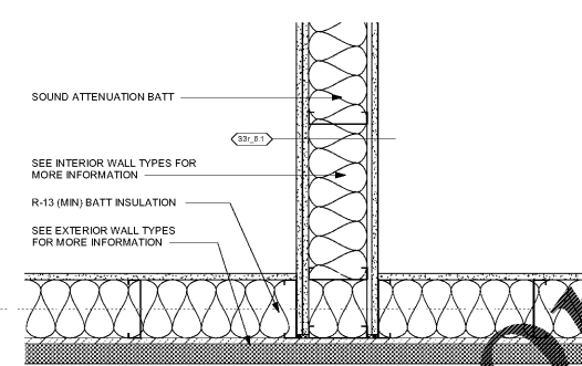
3 PD 2ND FLR TYP STUD TERMINATION @ EXTERIOR (EIFS) SCALE: 1 1/2" = 1'-0"
