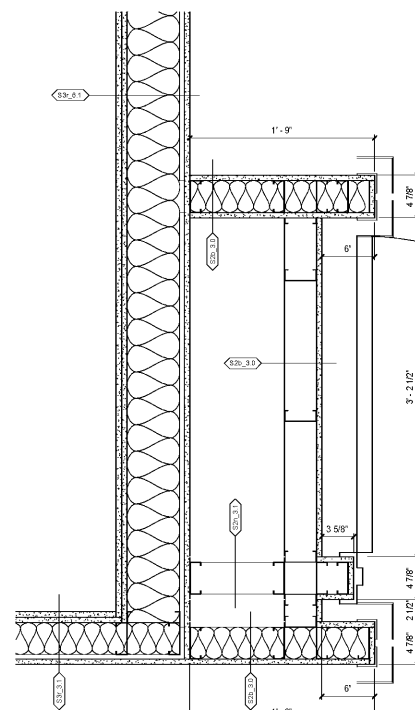
4 PD 2ND FLR B.4 (ELEV. LOBBY DOOR) SCALE: 1 1/2" = 1'-0"
