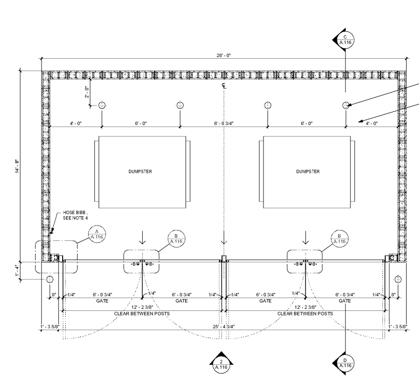
1 DUMPSTER ENCLOSURE PLAN SCALE: 3/8" = 1'-0"
