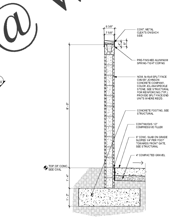
C DUMPSTER ENCLOSURE WALL SECTION SCALE: 3/4" = 1'-0"
