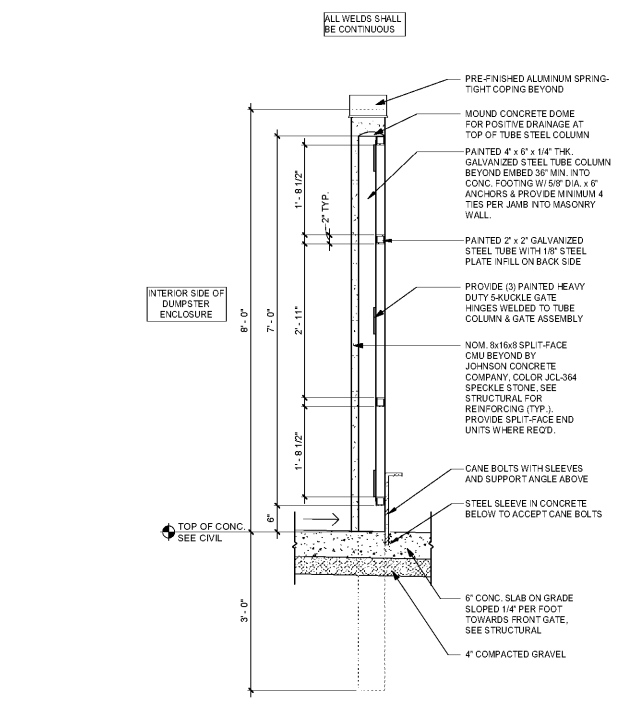
D DUMPSTER ENCLOSURE GATE SECTION SCALE: 3/4" = 1'-0"
