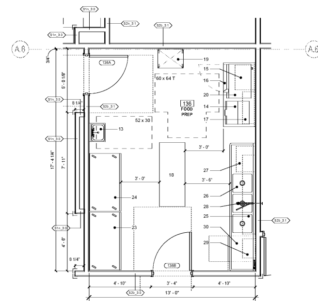
1 ENLARGED PLAN - FOOD PREP SCALE: 3/8" = 1'-0"
