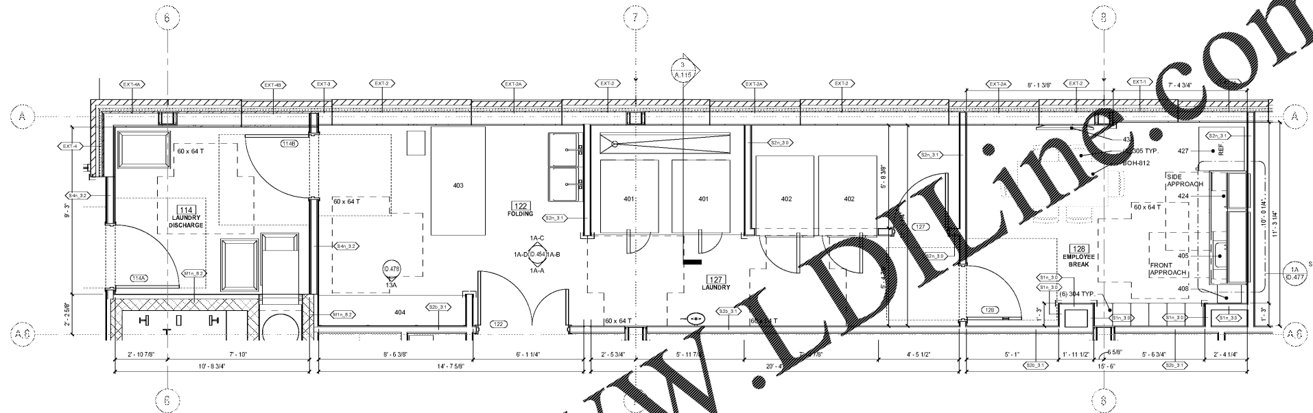
2 ENLARGED PLAN - LAUNDRY SCALE: 3/8" = 1'-0"
