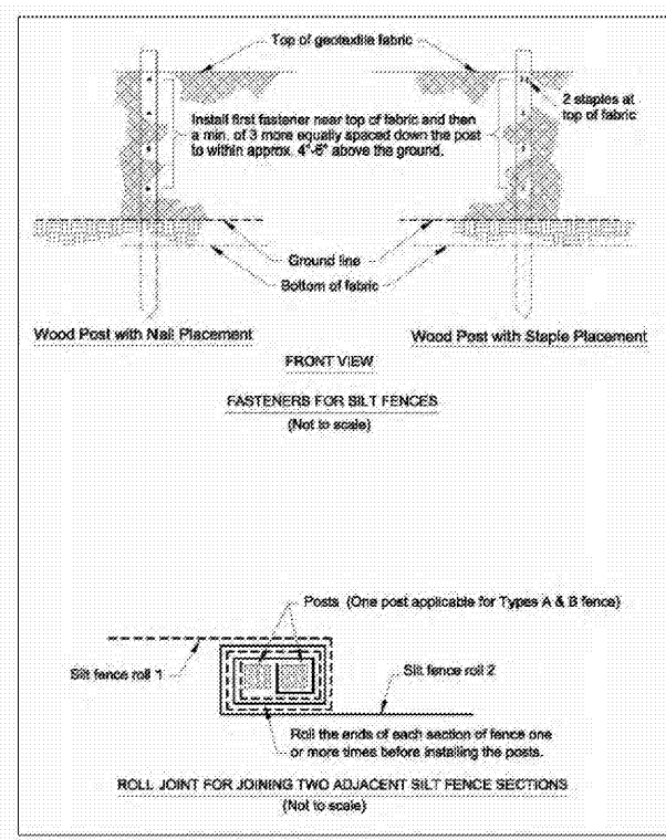
Figure SB-4 Silt Fence Installation Details
