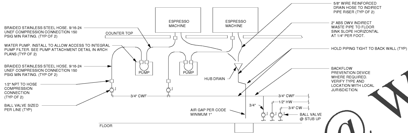
1 ESPRESSO MACHINE PIPING CONNECTION DETAIL Scale: NTS
