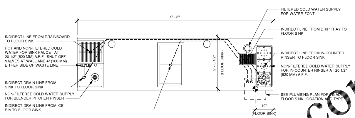
2 CBE 01-03 PLUMBING Scale: 3/4" = 1'-0"
