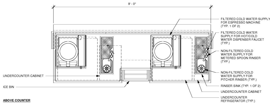
1 ESP 07-01 PLUMBING Scale: 3/4" = 1'-0"
