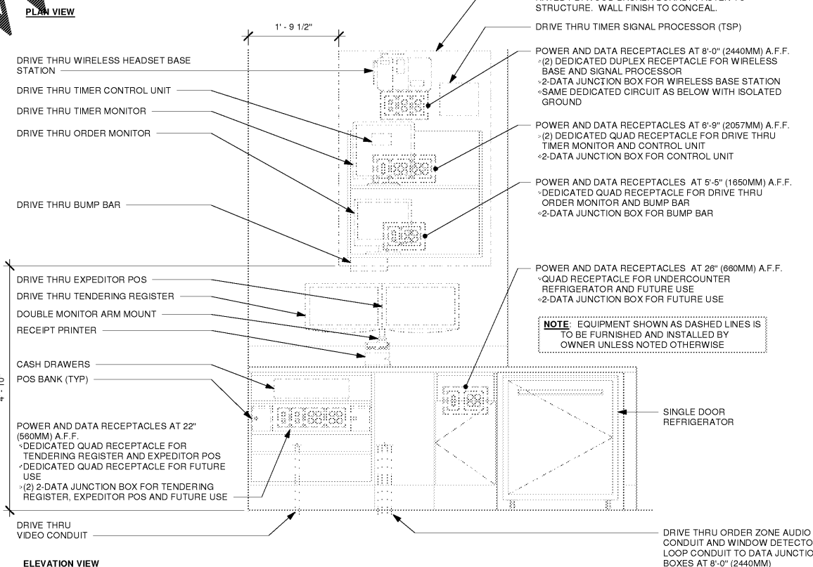
1 DTP 01-01 ELECTRICAL Scale: 3/4" = 1'-0"
