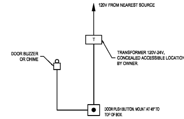
5 DOOR BELL DETAIL SCALE: NONE
