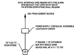
6 CARD READER DETAIL SCALE: NONE
