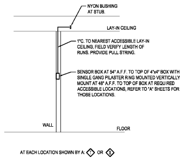
4 THERMOSTAT WALL BOX MOUNTING DETAIL SCALE: NONE
