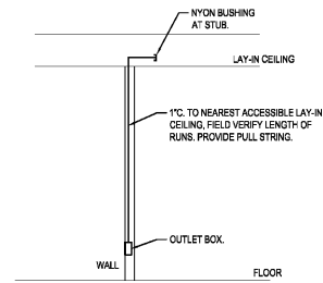
2 COMMUNICATION WALL OUTLET DETAIL SCALE: NONE
