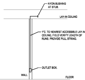
3 CATV WALL OUTLET DETAIL SCALE: NONE
