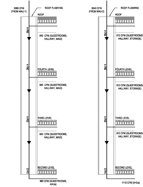
GROUND LEVEL (SA-1) SUPPLY AIR SHAFT
