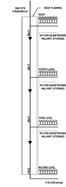
GROUND LEVEL (SA-2) SUPPLY AIR SHAFT
