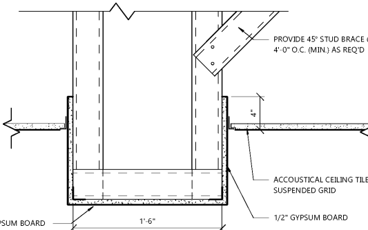
SOFFIT DETAIL NOT TO SCALE -SEE SHEET S1.1
