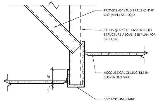
BULKHEAD DETAIL NOT TO SCALE *NOT REFERENCED ON PLANS
