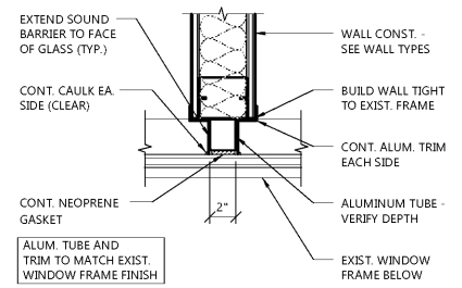
8 WALL CLOSURE DETAIL A5.1 NOT TO SCALE
