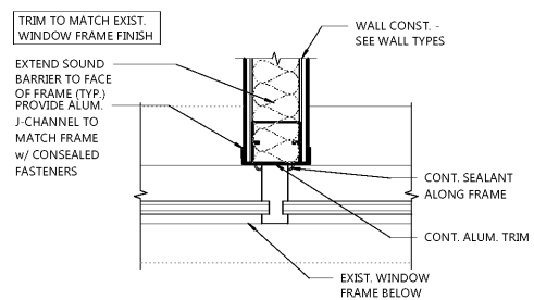
9 WALL CLOSURE DETAIL A5.1 NOT TO SCALE
