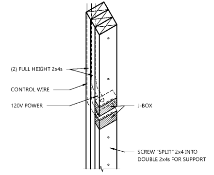
6 PASS THRU X-RAY ISOMETRIC A5.1 NOT TO SCALE
