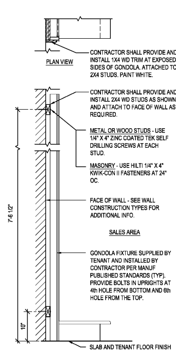
TYPICAL FIXTURE ATTACHMENT DETAIL SCALE: 1" = 1'-0"
