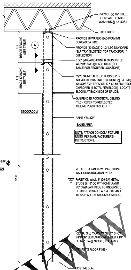
2 WALL SECTION - CONSTRUCTION TYPE: 5 SCALE: 1" = 1'-0"
