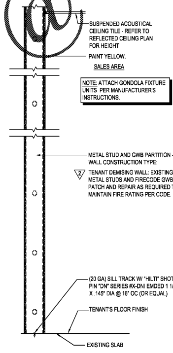
4 WALL SECTION - CONSTRUCTION TYPE: 2 SCALE: 1" = 1'-0"
