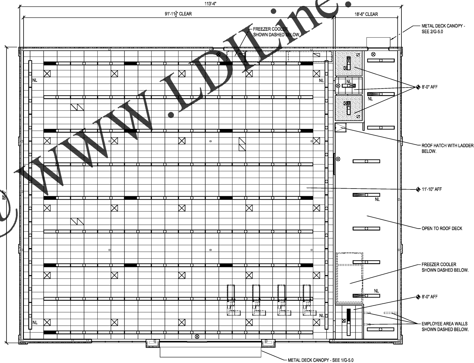
REFLECTED CEILING PLAN SCALE: 1/8"=1'-0"
