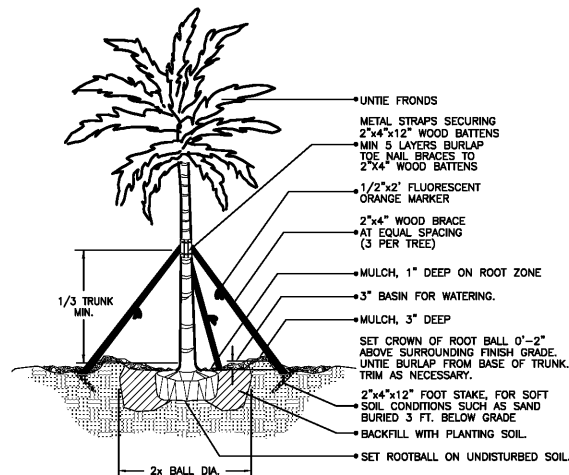
LARGE PALM PLANTING DETAIL
