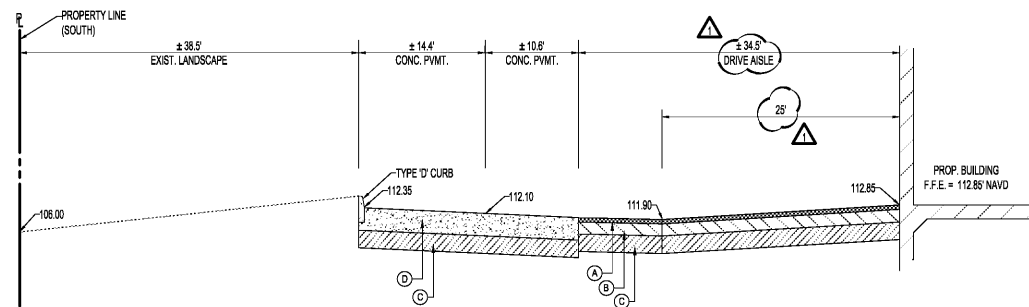
SECTION F-F
