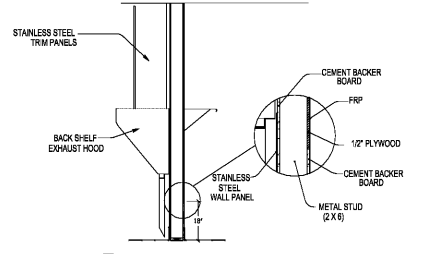
3 COOK LINE WALL SECTION FS-8.0
