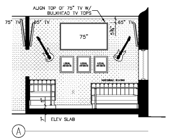
ELEVATED SIDE DINING ROOM ELEVATIONS SCALE: 1/4" = 1'-0"
