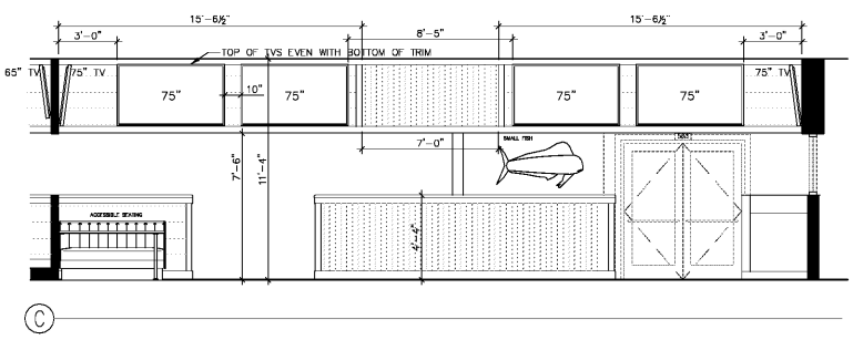
MAIN DINING ROOM ELEVATIONS SCALE: 1/4" = 1'-0"
