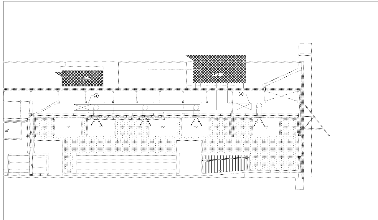
1 SECTION – SUPPLY AIR SYSTEM M5 SCALE: NONE
