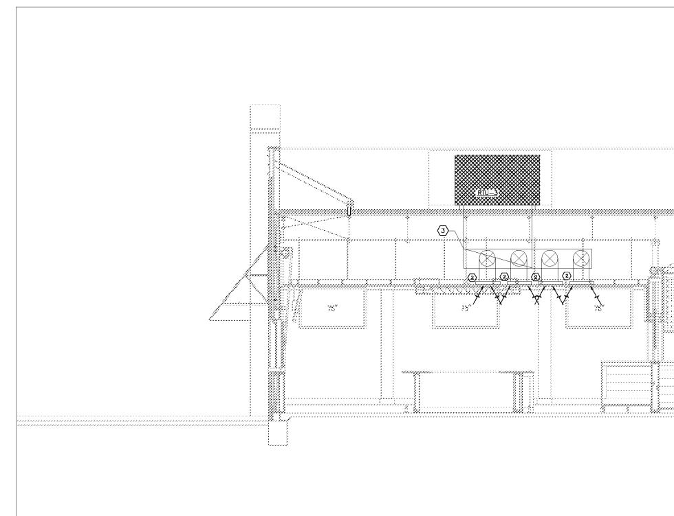
4 SECTION – RETURN AIR SYSTEM M5 SCALE: NONE
