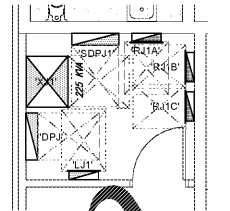
Enlarged Electrical Floor Plan Electrical Room J114
