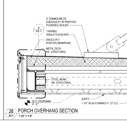
28 PORCH OVERHANG SECTION A3.1 1 1/2' x 1'-0"
