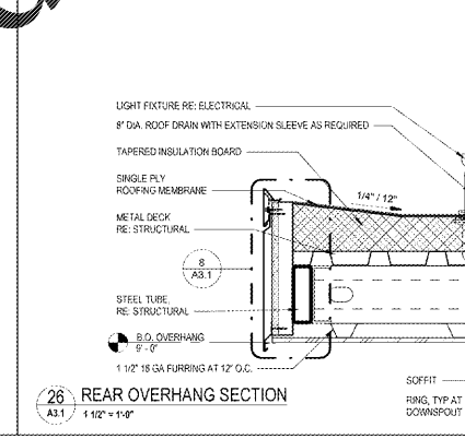
26 REAR OVERHANG SECTION A3.1 1 1/2' x 1'-0"
