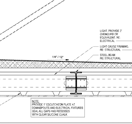
17 PARAPET DETAIL A3.1 2' x 1'-0"
