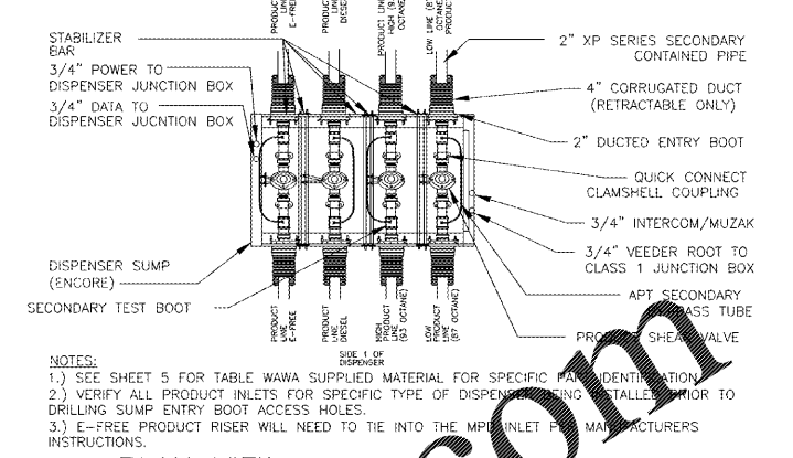
(G) PLAN VIEW DISPENSER SUMP - INLINE (3+1) G-3 SCALE: 3/4" = 1'-0"
