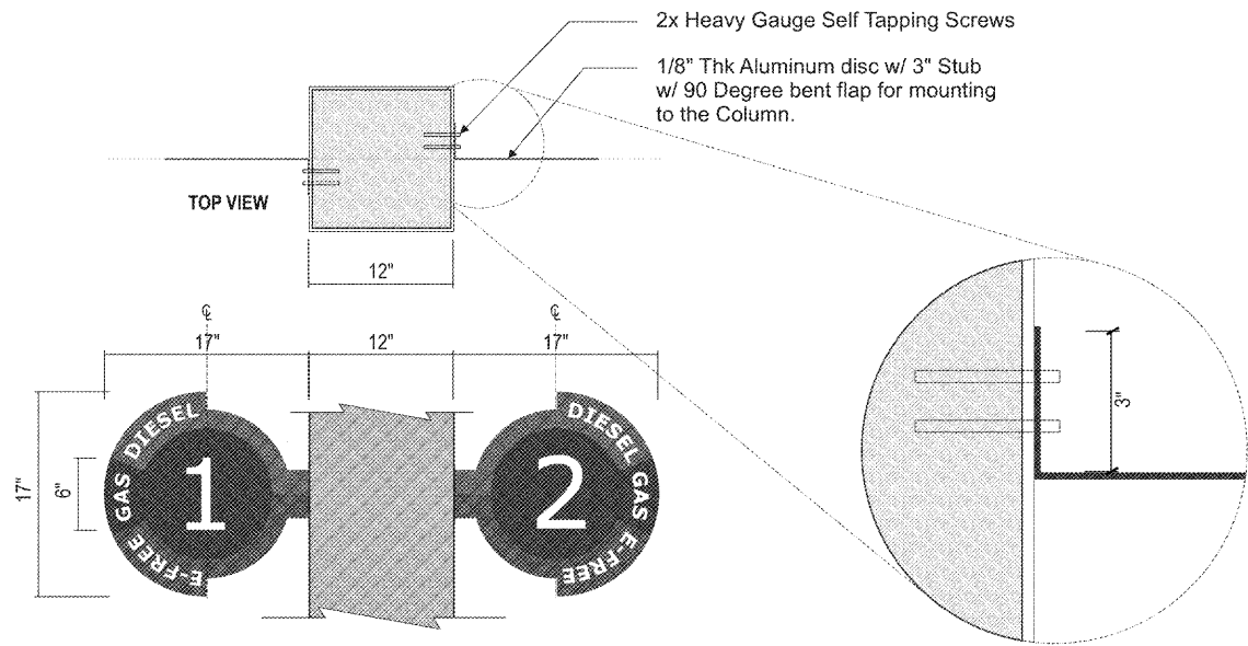
F PUMP NUMBERS (NON-ILLUMINATED) @ GAS PUMP CANOPY QTY: 12 (1 each) STANDARD SPECS - SEE COLOR SPECIFICATION LIBRARY SCALE: 1 1/2"=1'-0"
