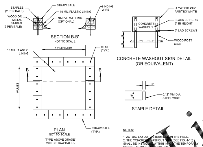
Cw CONCRETE WASHOUT NOT TO SCALE
