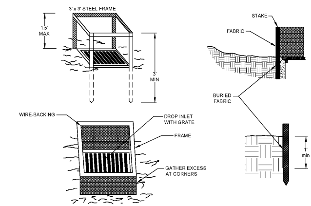
FIP INLET SEDIMENT TRAP - FILTER FABRIC WITH SUPPORTING FRAME NOT TO SCALE
