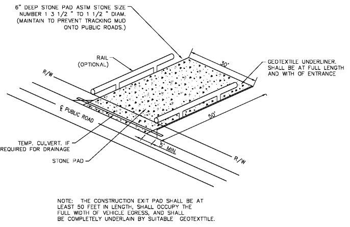
CEP CONSTRUCTION EXIT PAD NOT TO SCALE
