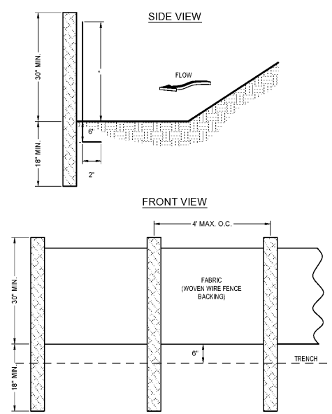
Sb SILT FENCE -TYPE SENSITIVE NOT TO SCALE
