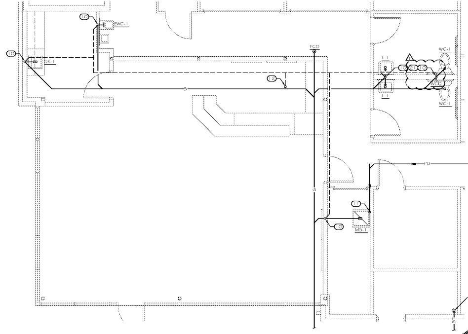
3 ENLARGED PLAN - WASTE & VENT P1.1 SCALE: 1/4"=1'-0"
