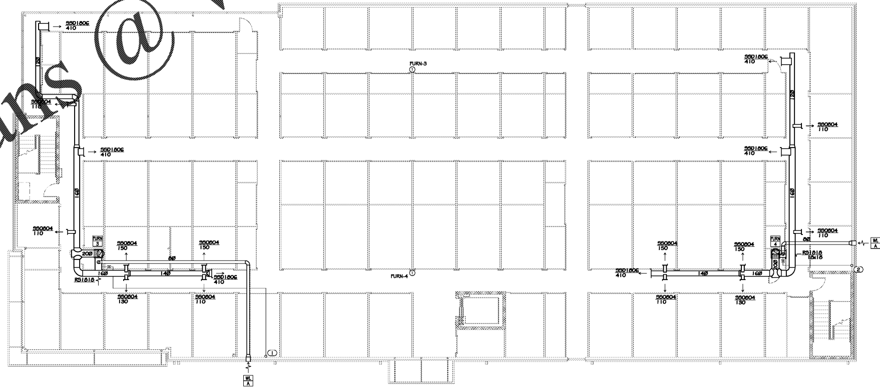
1 SECOND FLOOR PLAN M1.2 SCALE: 1/8"=1'-0"
