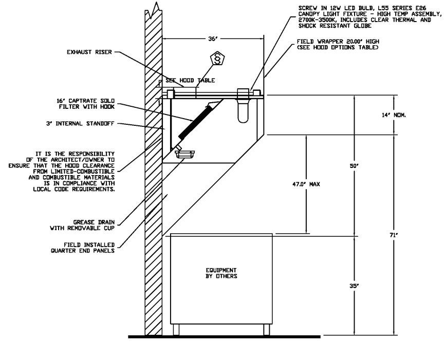
SECTION VIEW - MODEL 3650BD-2 HOOD - #4 (FRYER)
