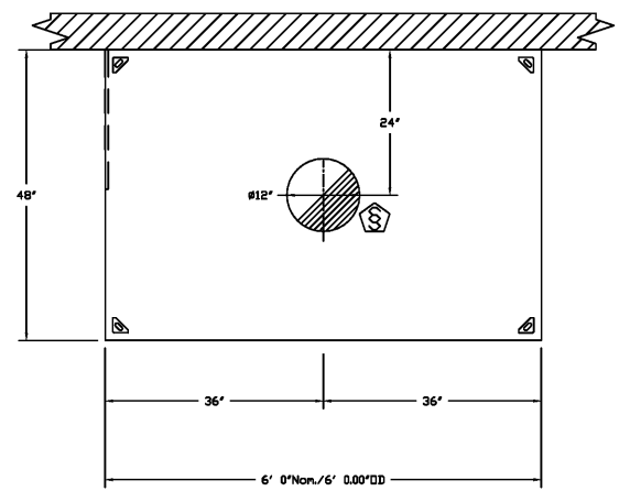
PLAN VIEW - Hood #5 (DISH) 6' 0.00" LONG 4824VHB-G
