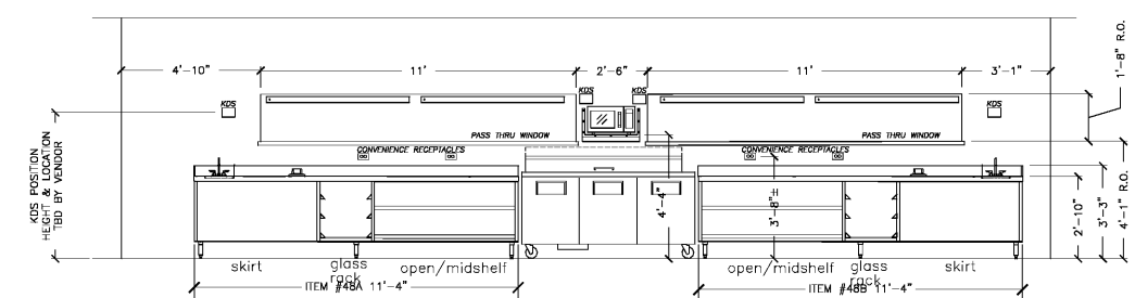
ELEVATION SERVICE AREA 3 3/8" = 1'-0"
