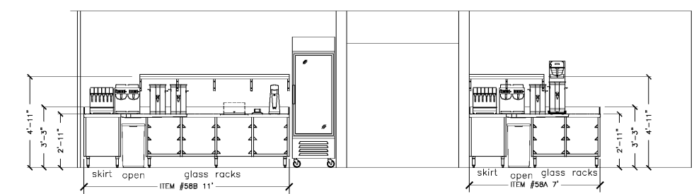
ELEVATION SERVICE AREA 4 3/8" = 1'-0"
