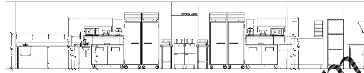
ELEVATION COOKLINE 1 3/8" = 1'-0"
