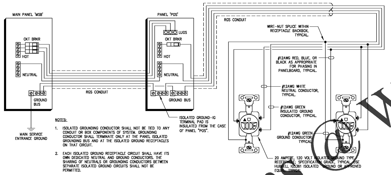
DEDICATED ISOLATED GROUND SCHEMATIC 4 NOT TO SCALE
