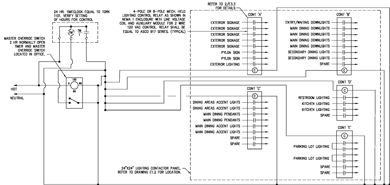
LIGHTING CONTROL DIAGRAM 1 NOT TO SCALE
