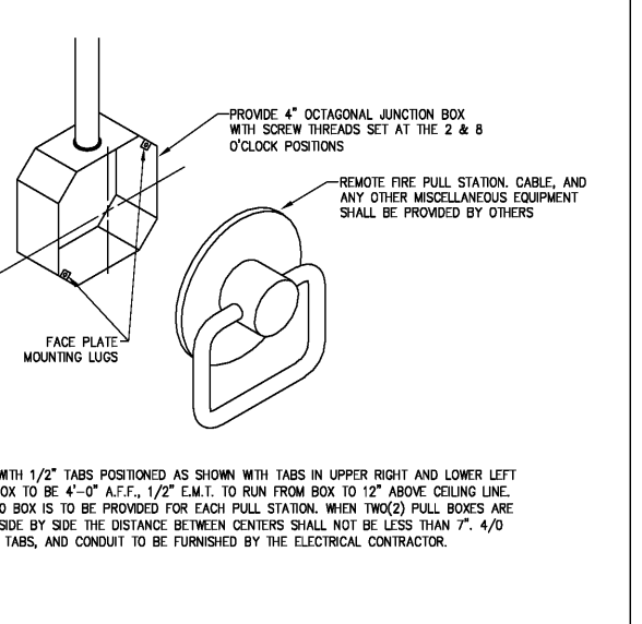
ANSUL PULL STATION DETAIL 6 NOT TO SCALE
