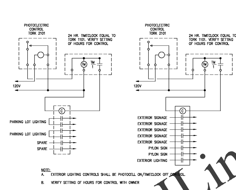
LIGHTING CONTROL DIAGRAM 2 NOT TO SCALE
