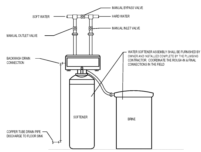
WATER SOFTNER DETAIL SCALE: NONE 7
