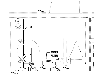
PLUMBING FLOOR PLAN - HOT, COLD, & GAS
