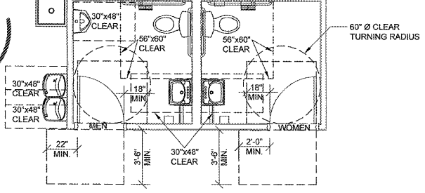
15 FLOOR SPACE CLEARANCES DIAGRAM A4.1 SCALE: 1/4" = 1'-0"
