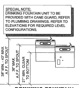
16 DRINKING FOUNTAIN CLEARANCES A4.1 SCALE: 1/2" = 1'-0"
