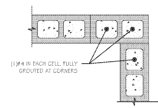
5 PLAN VIEW SD-2 SCALE: 1" = 1'-0"
