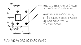
PLAN VIEW: BP8 10 BASE PLATE
