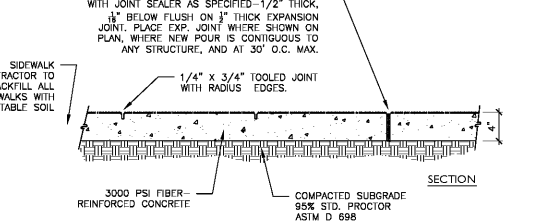
5 Exposed Aggregate Concrete Sidewalk Detail N.T.S.
